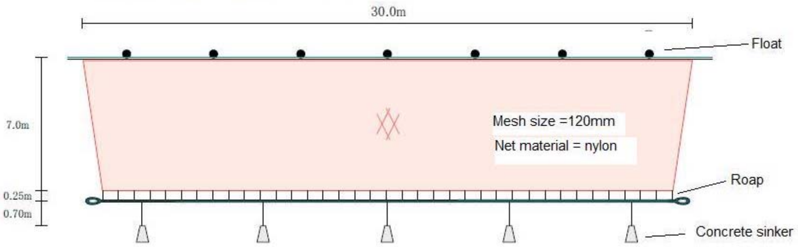
Structure of a net panel (tan in Japanese)
