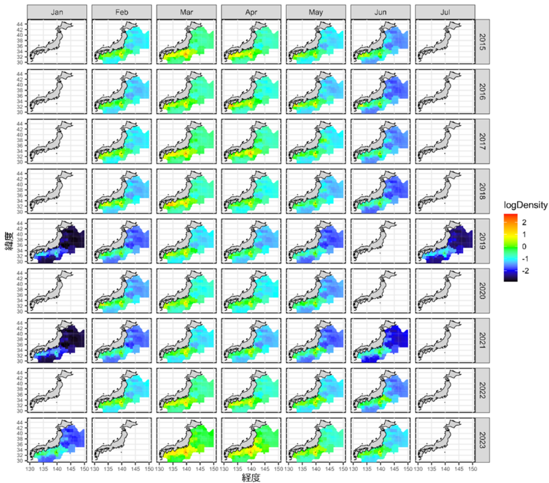
Figure 3: Spatial distributions of blue mackerel eggs on the Pacific coast of Japan by month (column) by year (row), estimated from the seasonal VAST model (Thorson et al. 2020) with the egg survey data. The sign of X in red represents the center of gravity.
